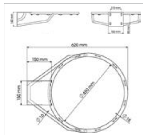
S14335 O Standard ring with 4 reinforcements
